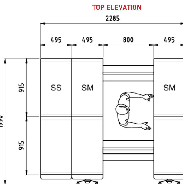
6 BAYS WITH 2 BAYS DEEP OVERALL DIMENSIONS : 2285 W x 1990 D x 2215 H MM
